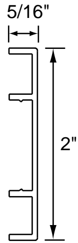
304-2 Trim
